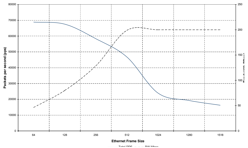
100 Mbps Bi-directional throughput for the Clavister S240
